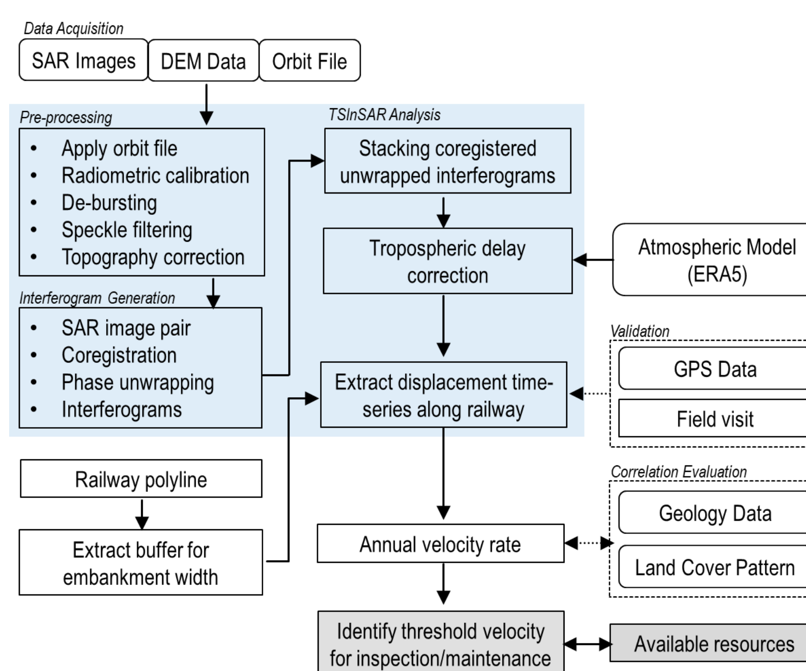
Fig1. Research Framework.
